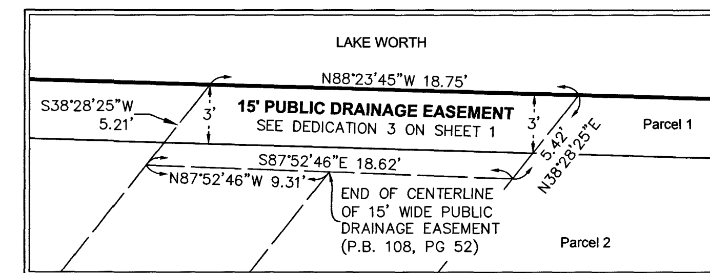
DETAIL "B" 1" = 5'
